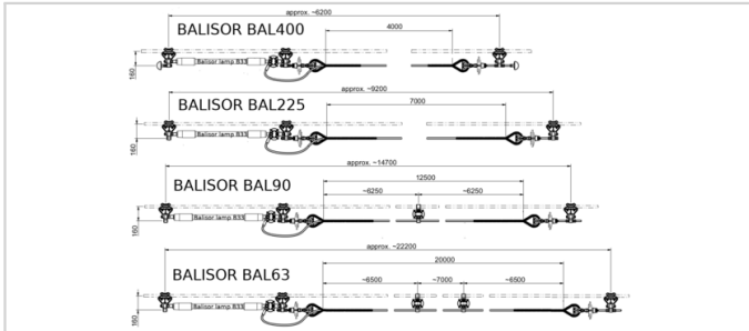
Length of the drift depending on the voltage
