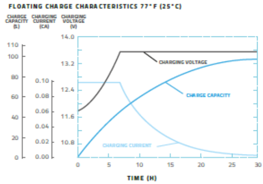
FLOATING CHARGE CHARACTERISTIC (25°C)
