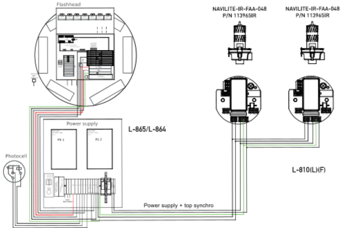
L-864 & L-865/L-864 OBSTAFLASH OFP/OFI 120/240Vac with L-810(L)(F)
