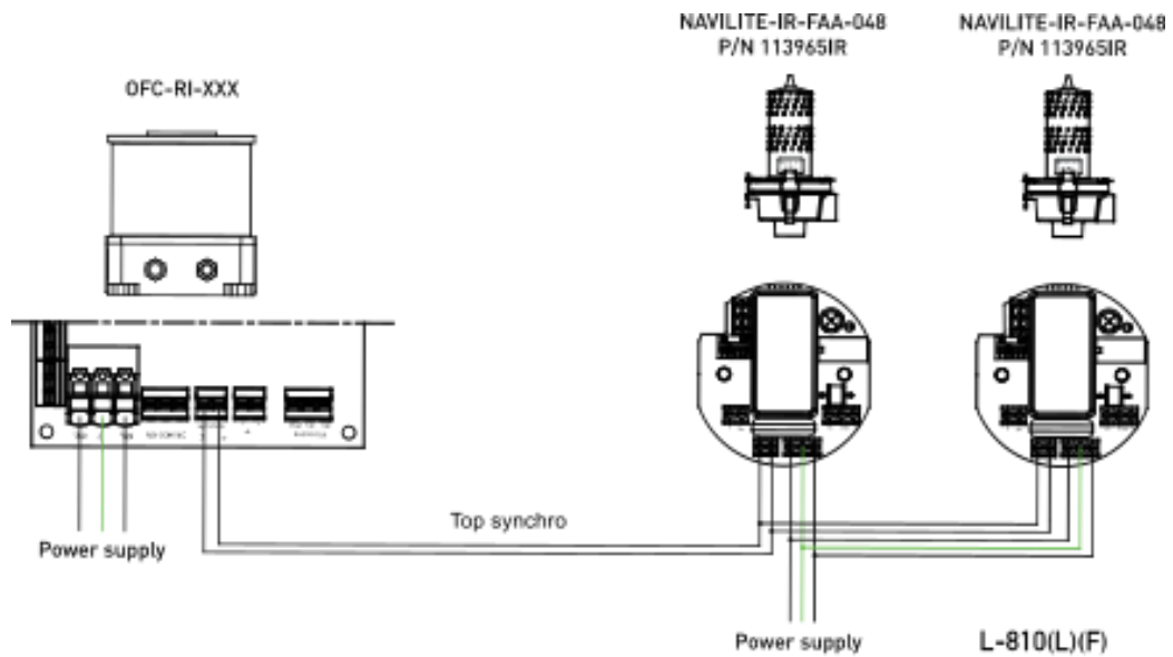
L-864 with L-810(L)(F)
