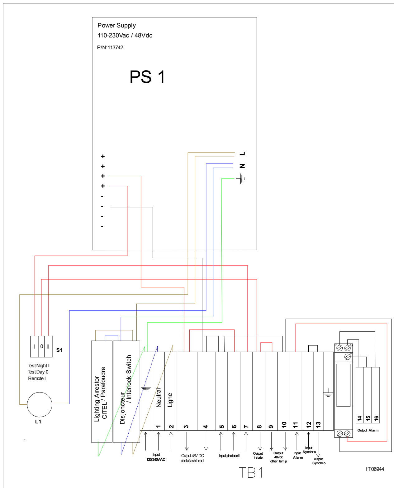
Figure 2-3. INTERNAL WIRING DIAGRAM OF POWER SUPPLY P/N113797
