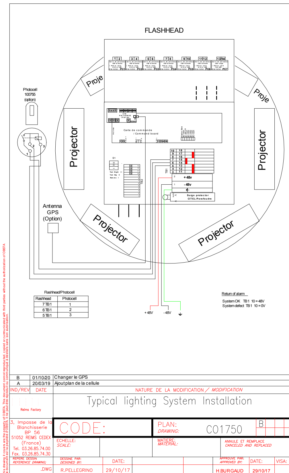
Figure 2-7. WIRING DIAGRAM OF flash-head P/N113792 + PHOTOCCELL 100755
