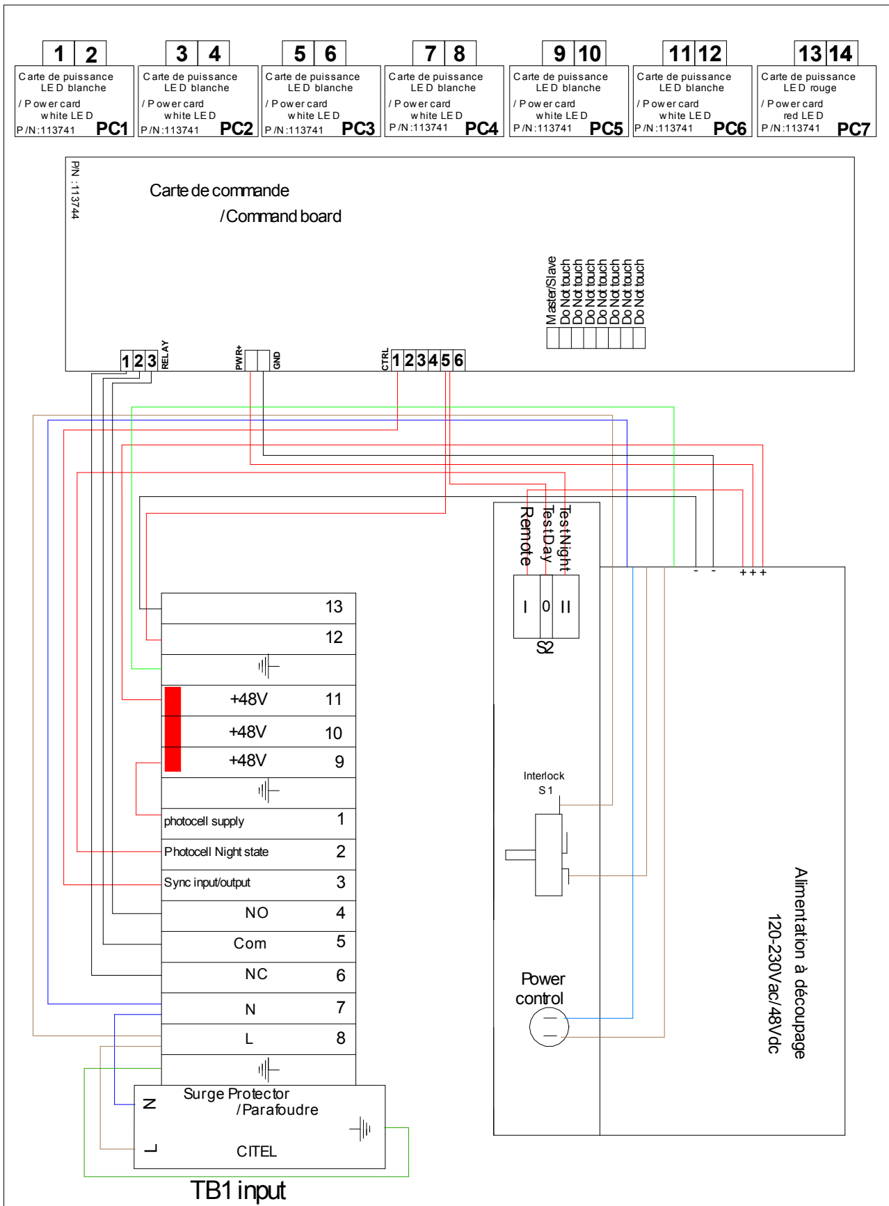
Figure 2-2. INTERNAL WIRING DIAGRAM OF POWER SUPPLY P/N113733
