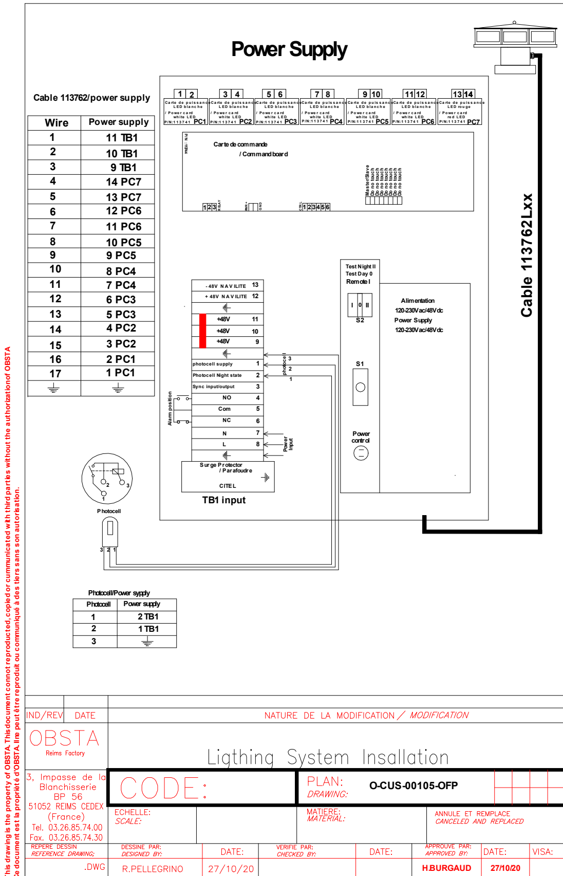
Figure 2-1. WIRING DIAGRAM OF OBSTAFLASH
