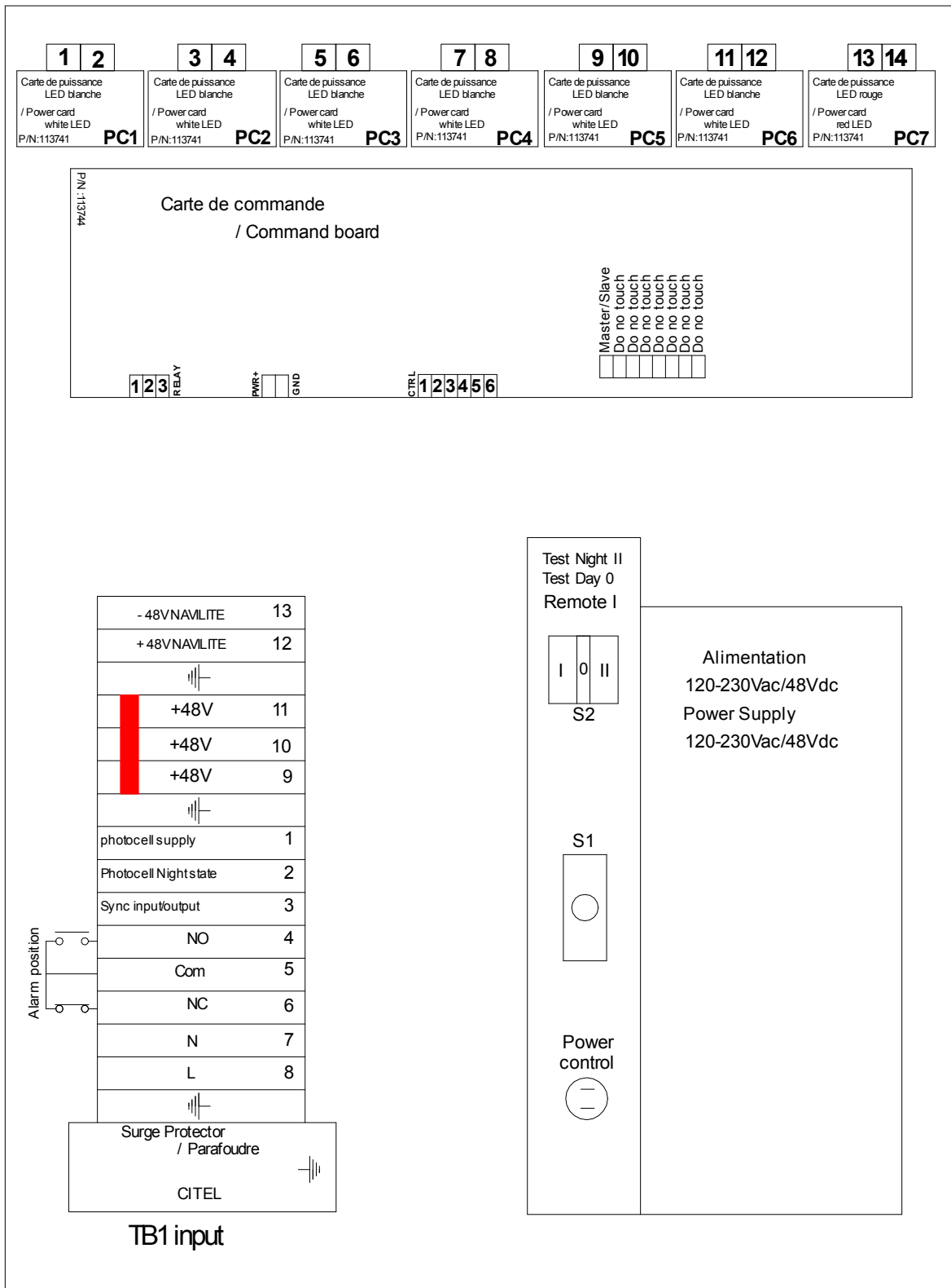
Figure 1-2. POWER SUPPLY COMPONENT LOCATIONS P/N 113733
