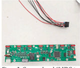
Figure 2: Command card 48 VDC + TORON CMD 12 PTS
