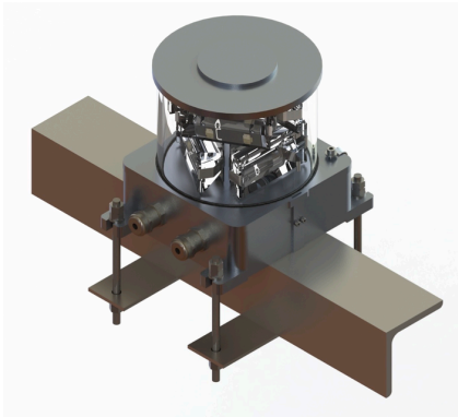
OFC bracket for horizontal bracket
